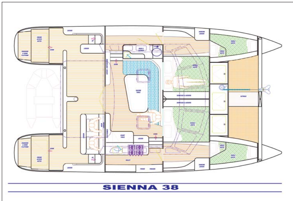
Below deck layout of Cruczar. Sleeping 8 adults.
